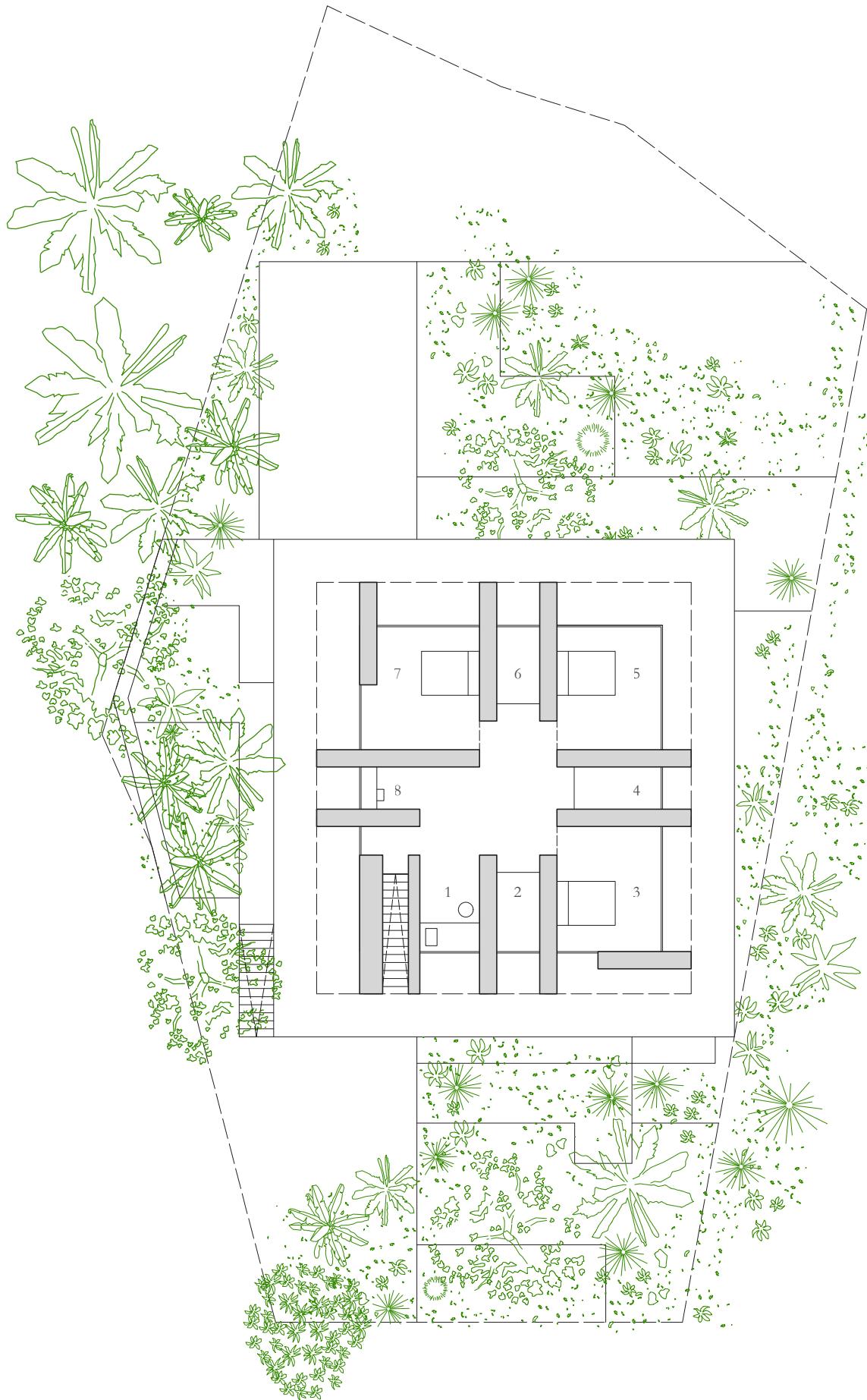
Upper Floor 1:200
