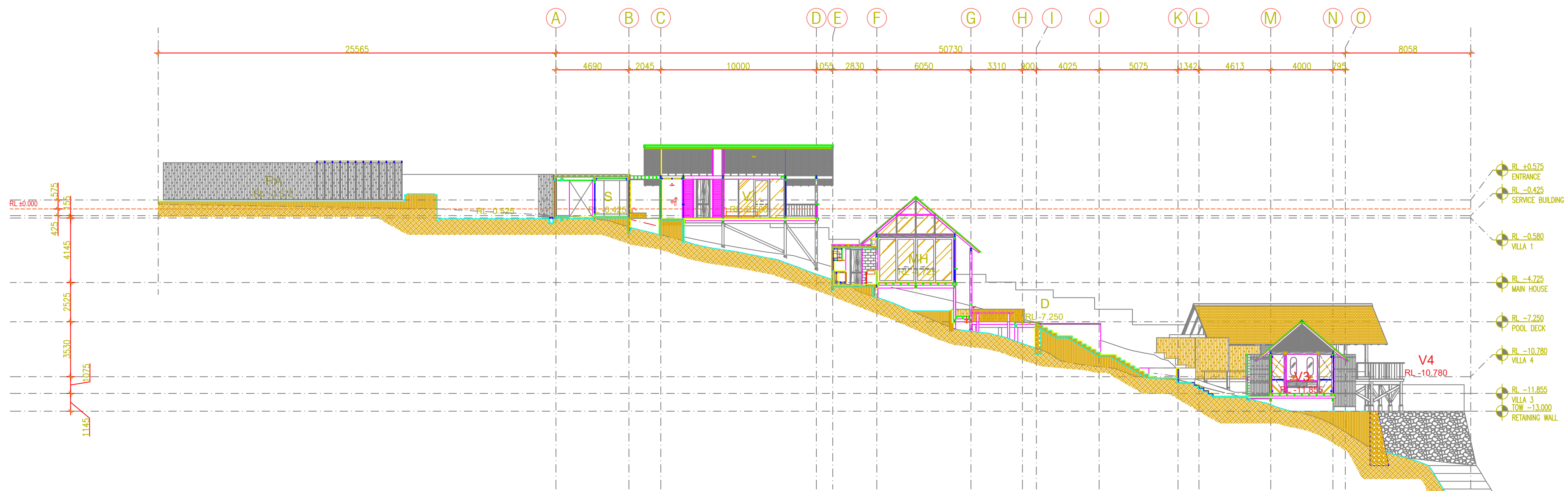
C SECTION A.00-100 SCALE 1:200 @A2
